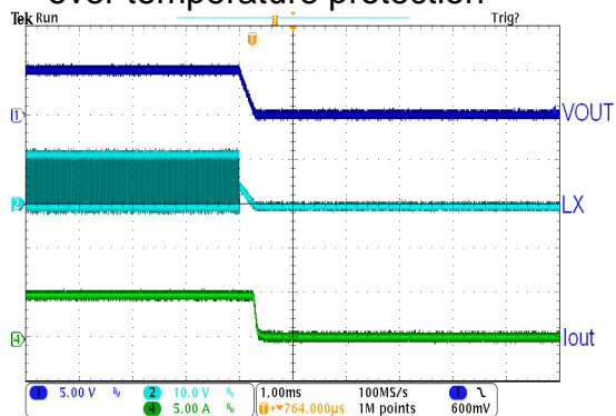
12Vin to 5Vout/4.8A load over temperature protection
