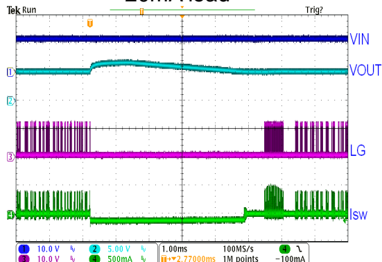
over voltage protection 20mA load
