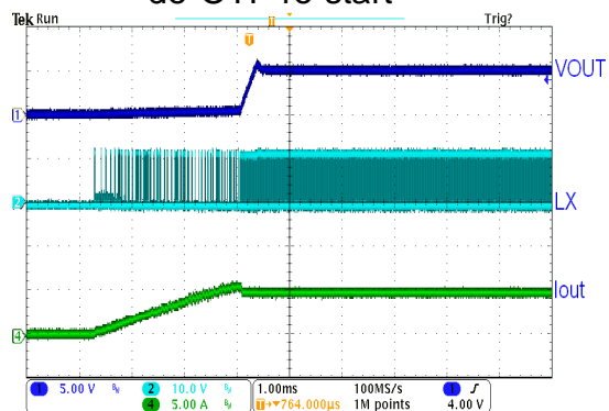
12Vin to 5Vout/4.8A load de-OTP re-start
